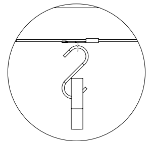
Twist Clip Loop on ceiling grid with S-hook through Zintra
