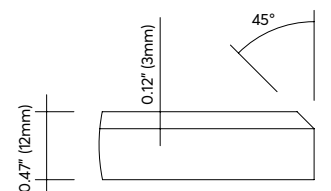
Typical Edge Detail
